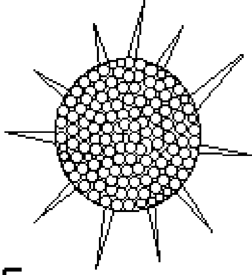
A radiolarian
