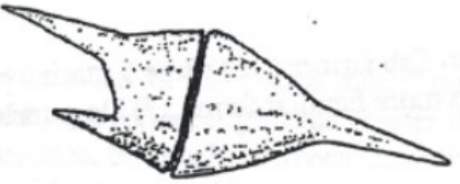
89 Ceratium lineatum
